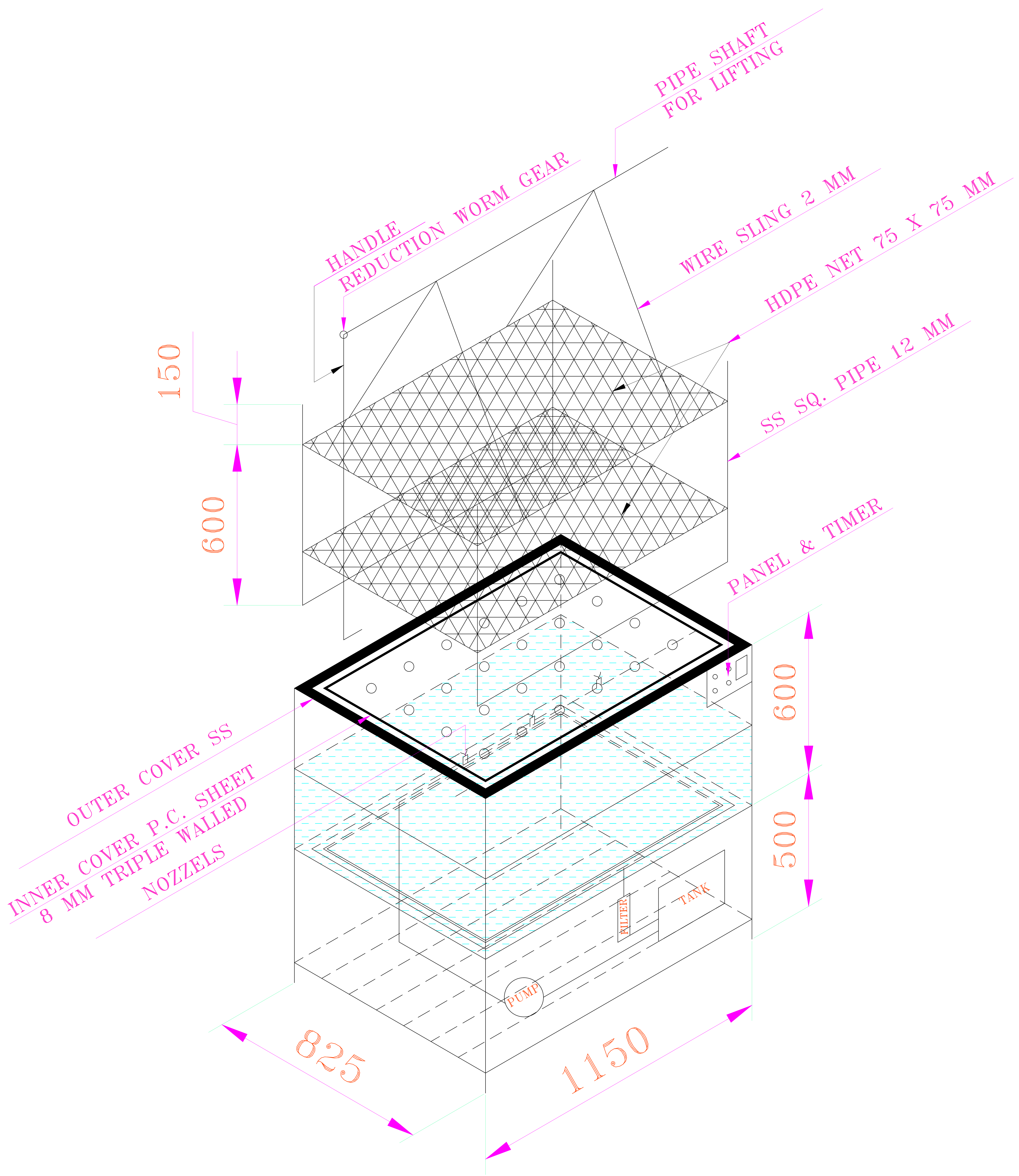
ISOMETRIC VIEW
